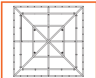
SMALL NET SIZE: 2460 X 2460MM
