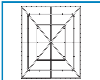
LARGE NET SIZE: 2800 X 3440MM
