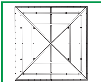
MEDIUM NET SIZE: 2800 X 2840MM
